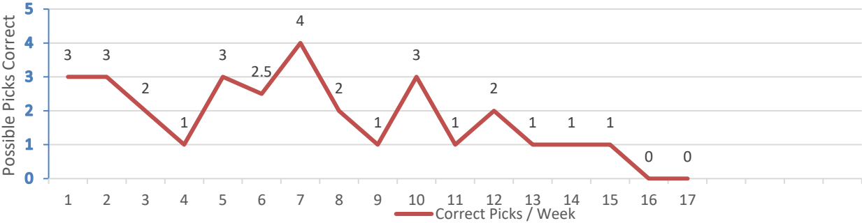
GA CONSORTIUM NUMBER OF PICKS CORRECT BY WEEK
